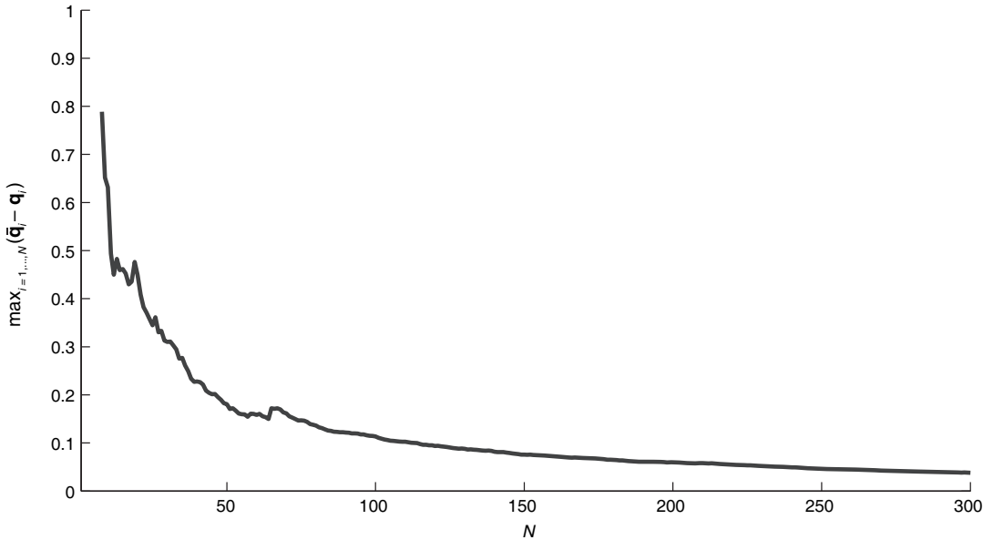
Fig. 4. Largest margin \max_{i=1,\dots,N}(\bar{q}_i - q_i) of example 2 as a function of N
