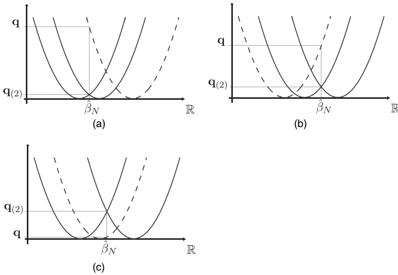
Fig. 8. The three parabolas (---, (Y - \beta)^2 ; —, parabolas corresponding to the data set D^2 ): (a) q > q_{(2)} ; (b) q > q_{(2)} ; (c) q \leq q_{(2)}
