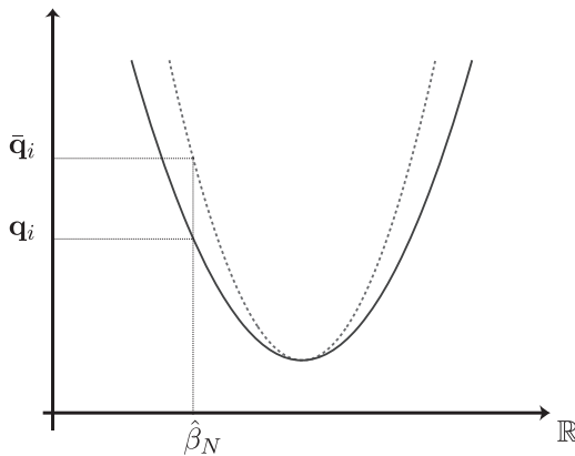
Fig. 2. The paraboloid (\beta - v_i)^T K_i (\beta - v_i) + h_i (—) versus the paraboloid (\beta - v_i)^T \bar{K}_i (\beta - v_i) + h_i with increased curvature (· · · · ·): their values at \beta = \hat{\beta}_N are the empirical cost \mathbf{q}_i and the modified empirical cost \bar{\mathbf{q}}_i respectively
